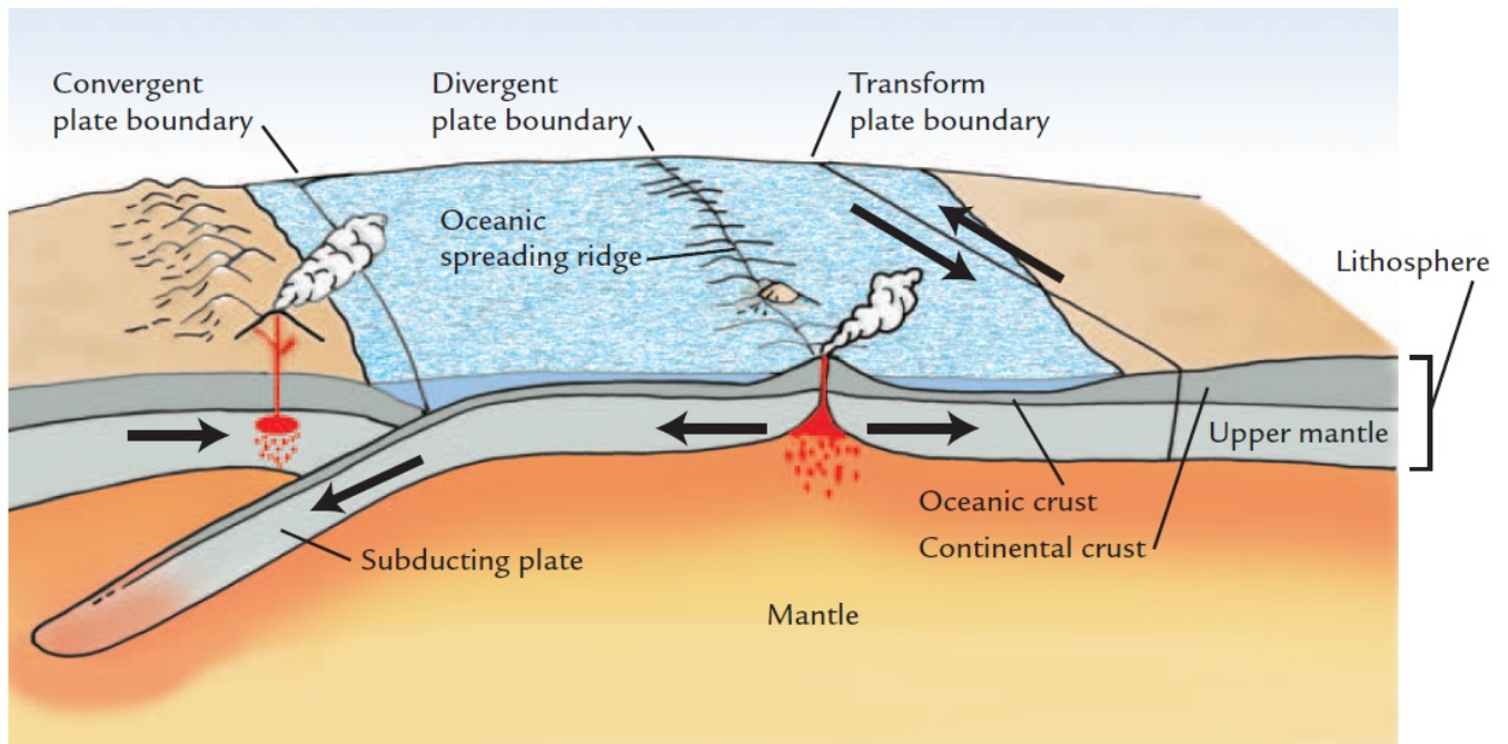
Figure 2: Types of Plate Boundaries
